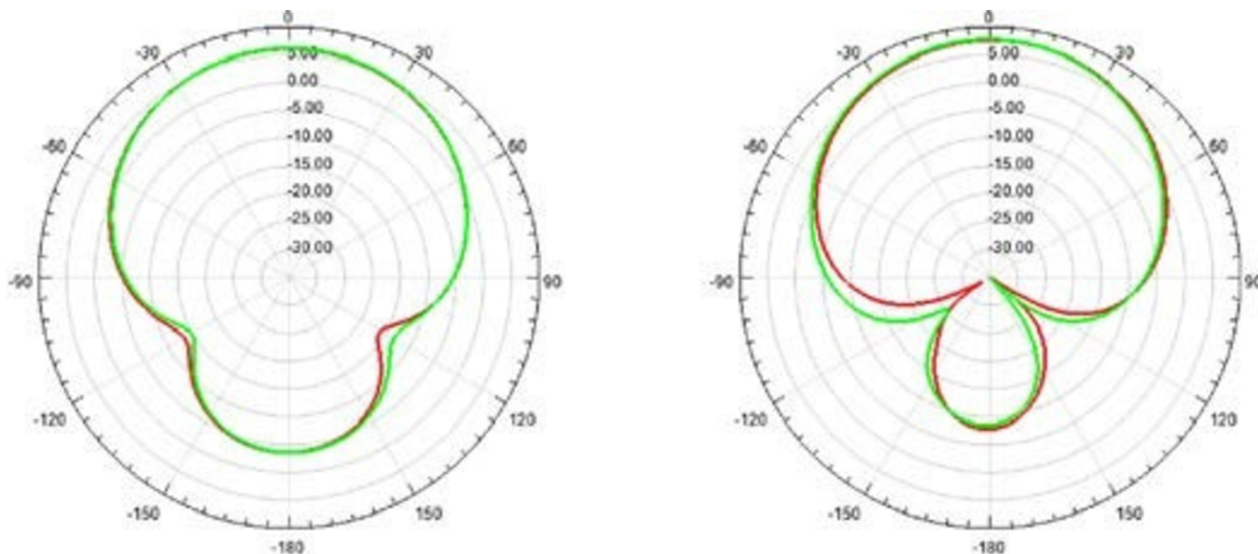
918MHz and 2.4GHz Radiation patterns
